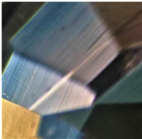
Figure 19: twinning in sample SW10. Darkfield and crossed polarizers – 60x magnification
