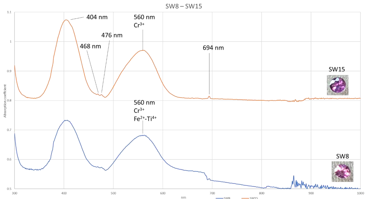
Figure 22: samples SW8 and SW15 have spectra dominated by \text{Cr}^{3+} . However, in SW8 the \text{Cr}^{3+} large band centred at 560 nm is stacked with \text{Fe}^{2+}\text{-O}^{2-}\text{-Ti}^{4+} which is not the case of SW15. No cut off after 300 nm for the two samples. Note in sample SW15 the two small peaks at ~468 and 476 nm due to iron, they are also present in a lot of spectra.
