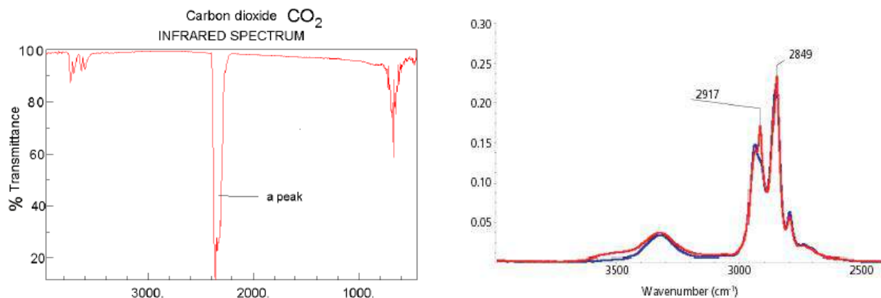
Figure 25: left – CO 2 peak (image taken from http://webbook.nist.gov/cgi/cbook.cgi?ID=C124389&Type=IR-SPEC&Index=1 ), right – peaks related to oil and fats contamination due to handling (image taken from https://www.azom.com/article.aspx?ArticleID=11722 )
