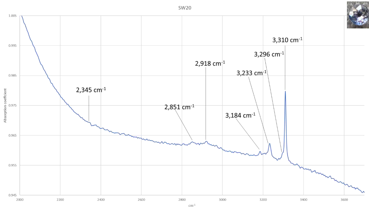
Figure 28: Sample SW20 showing OH related peaks at 3,184 – 3,233 – 3,296 – 3,310 cm -1 . The peaks are higher than in any other spectrum
