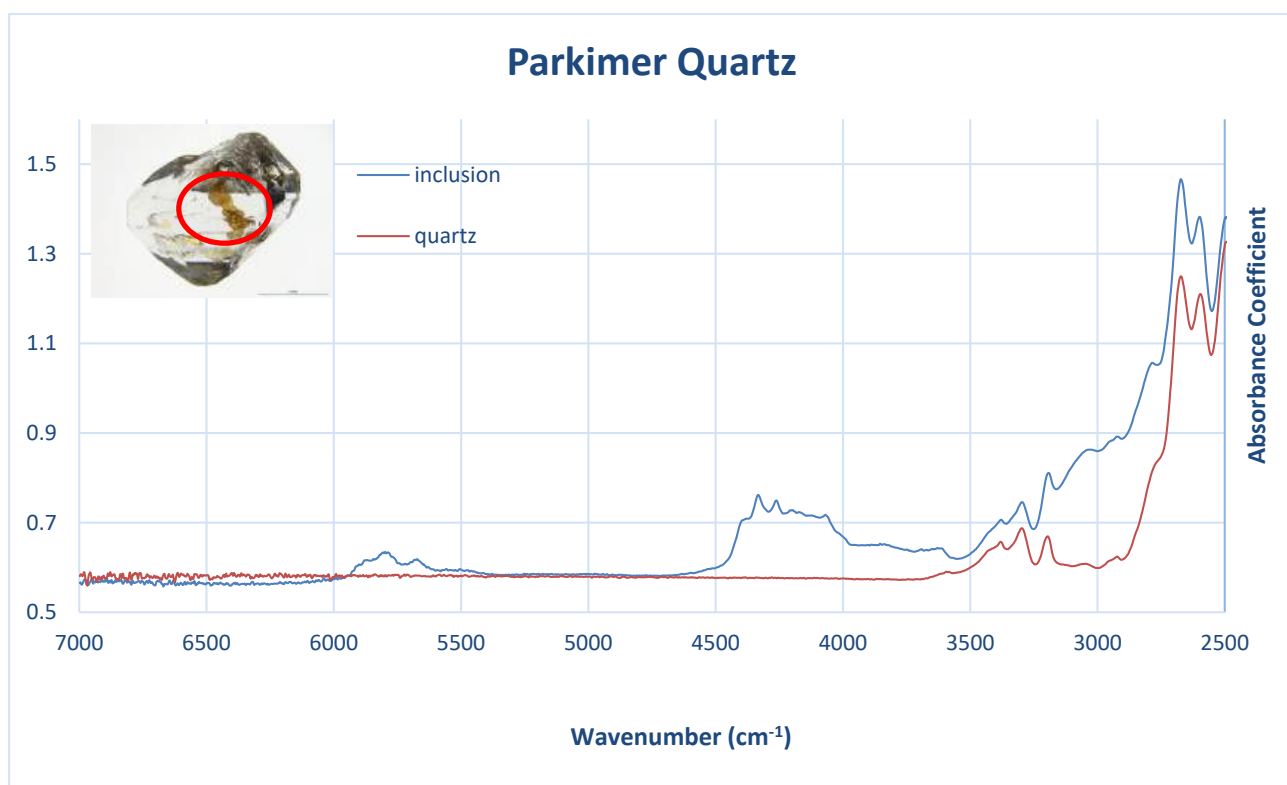
Figure 11: The yellow inclusion spectra show different peak from pure quartz in range 7000 to 3500 \text{cm}^{-1}
