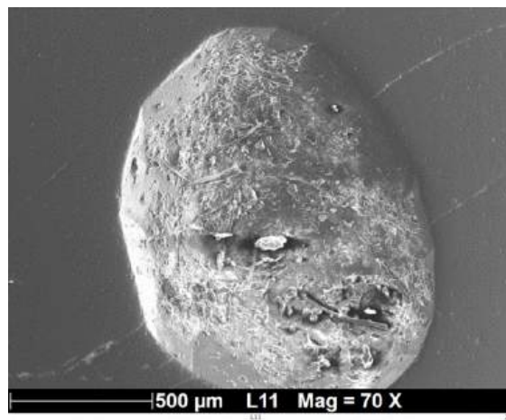
Figure 22: SEM photo of sample PD4 (secondary electrons)
