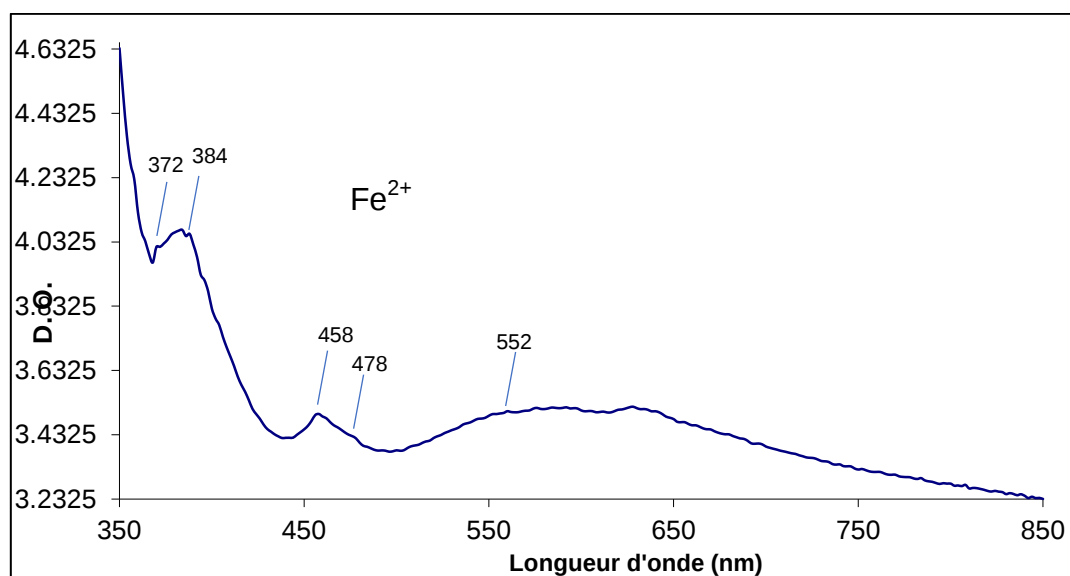
Figure 15: Isolated sample PD5 showing \text{Fe}^{2+} absorption spectra
