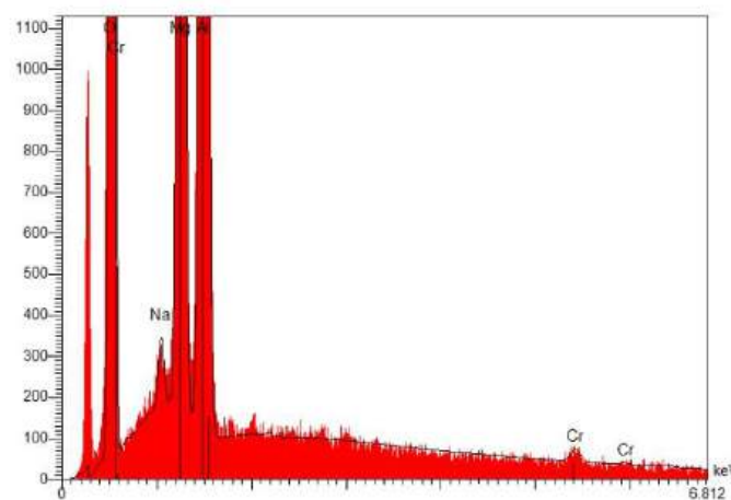
Figure 24 : SEM chemical spectra show Cr peak was obtained from PD 9 sample.
