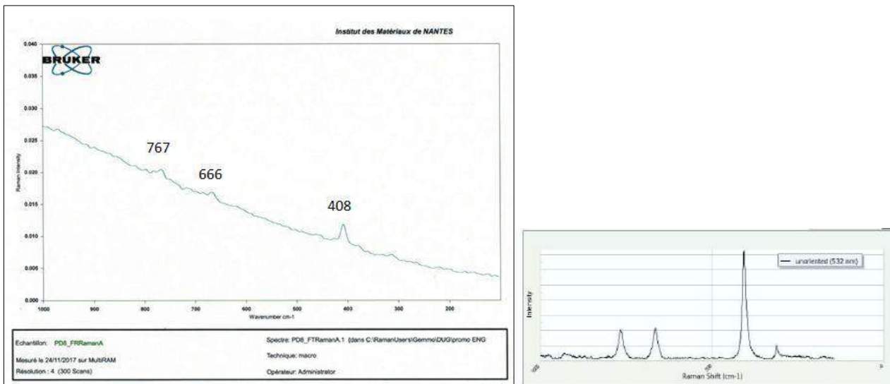
Figure 21: PD 8 sample shows raman shift at 408 , 666 and 767 cm-1 (left) which corresponds to the raman spectra from myanmese spinel of RRUFF ID: R050184 (right). ( http://rruff.info/Spinel/R050184 )
