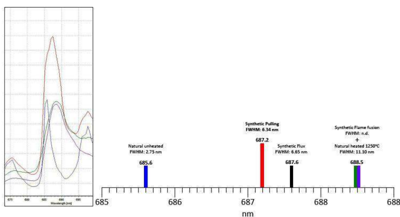
Figure 20 : The main band of \text{Cr}^{3+} luminescence positions are measured at the center at the band at half height showing the difference of FWHM of the unheated, heated and synthetic spinel samples. (Notari F, 2017)
