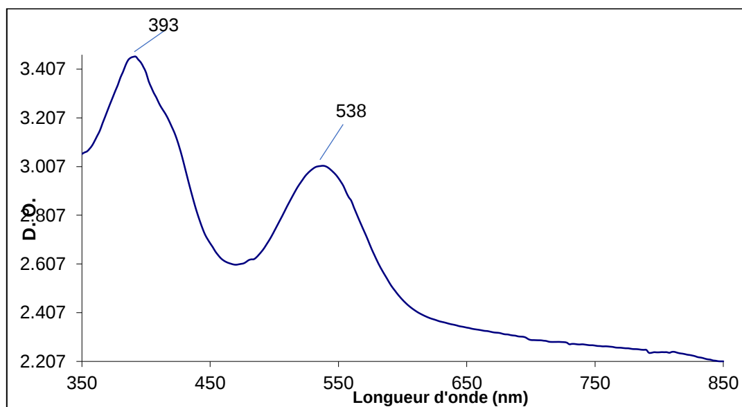
Figure 17: Isolated sample PD8 showing Cr 3+ absorption spectra
