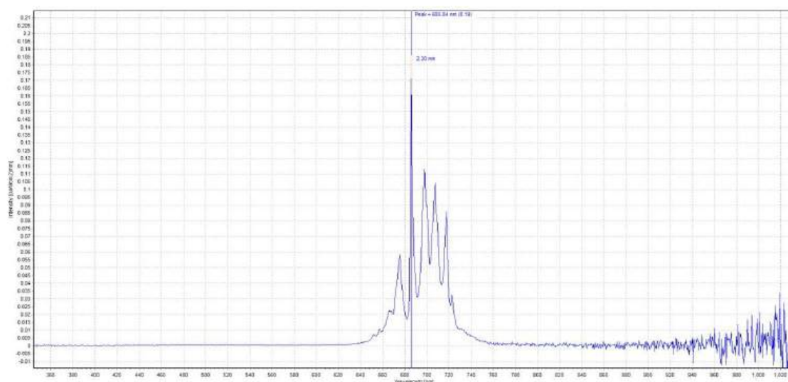
Figure 19 :Well-defined chromium emission features in the photoluminescence spectrum obtained from all 12 samples confirm they are all natural and unheated .
