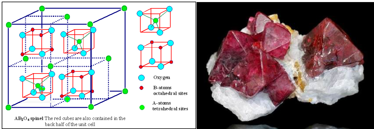
Figure 1 : Schematic of spinel structure (Deer, Howie and Zussman, 1996) ( https://nptel.ac.in/courses/113104005/lecture3/3_9.htm )
