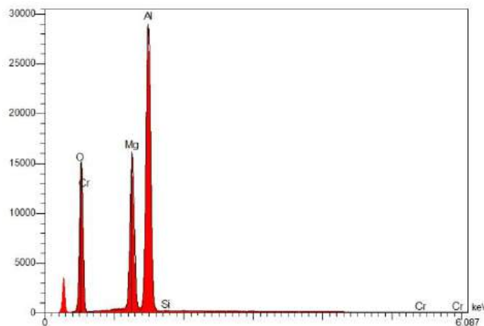
Figure 23 : SEM chemical spectra obtained from PD4, PD6, PD7, PD10 and PD11
