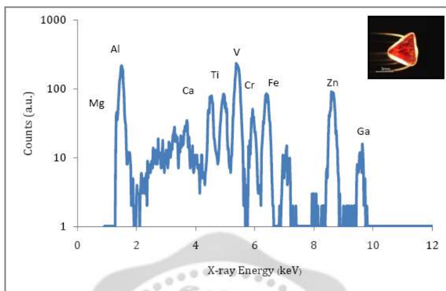
Figure 25: Spectrum obtained from PIXE technique of orange red spinel from Myanmar Srisataporn B. (2013)
